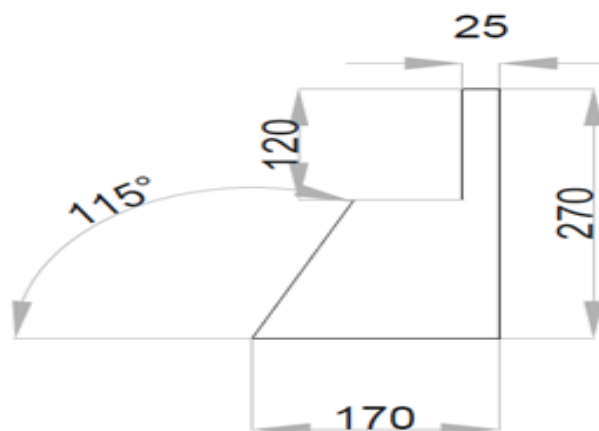
Fig. 9 Design of tiller (all dimensions in mm)
