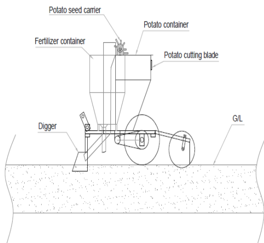
Fig. 16 Line Diagram of Potato Planting Machine
