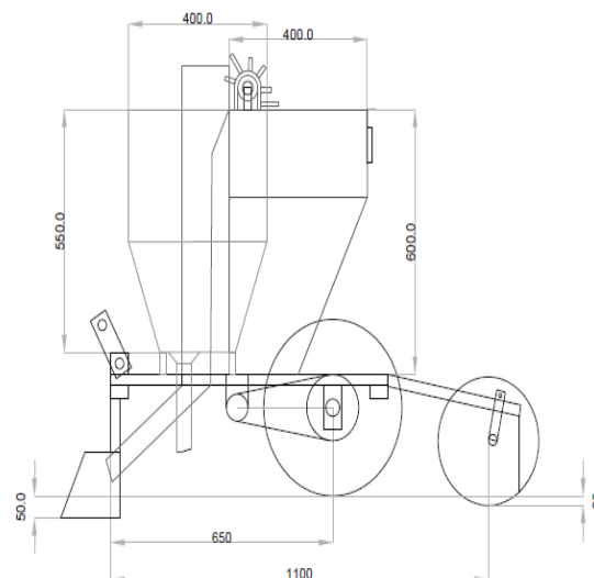
Fig. 17 Potato Planting Equipment With Dimensions
